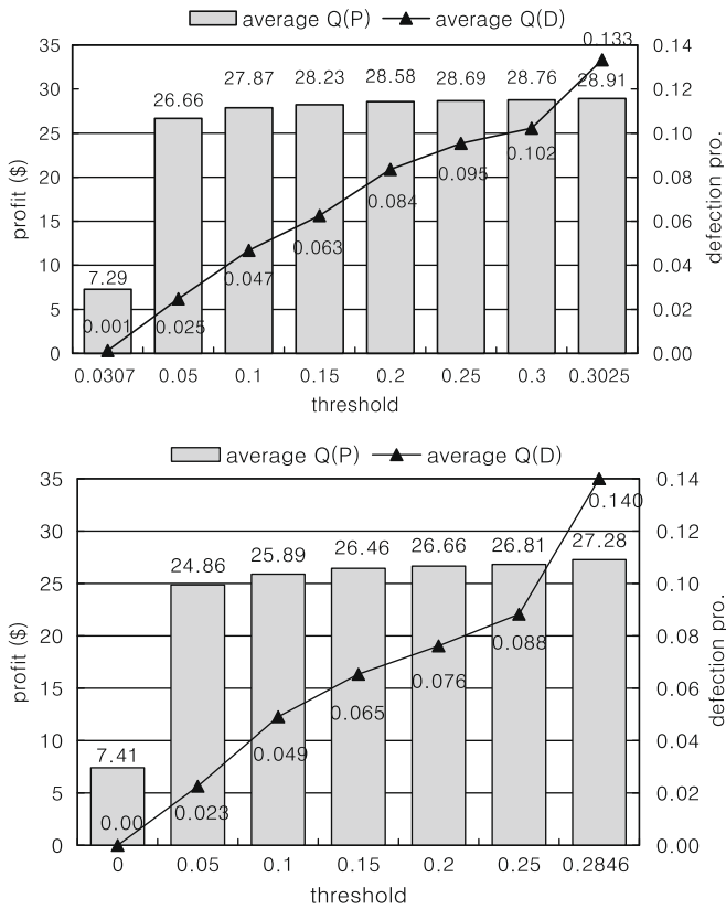
Fig. 4. Performance comparison of different thresholds. (a) Average Q_p and Q_d value in the 6 \times 8 SOM model; (b) Average Q_p and Q_d value in the 6 \times 7 SOM model.
