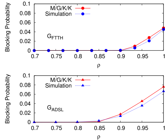
Fig. 1. Comparison of the blocking probability between analytical model and simulation when increasing the system load for G_{FTTH} (top) and G_{ADSL} (bottom).
