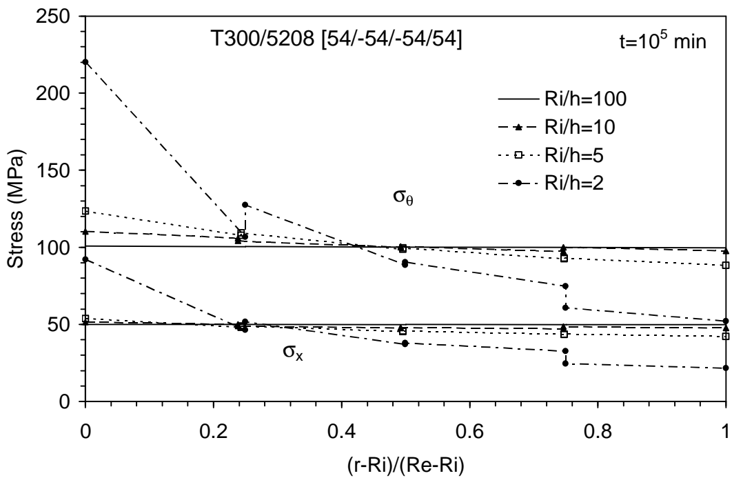
Figure 11: Axial and hoop stress distribution the instant t=10^5 min for cylinders [54/-54/-54/54] under internal pressure with inner radius to thickness ratios R_i/h of 100, 10, 5 and 2.
