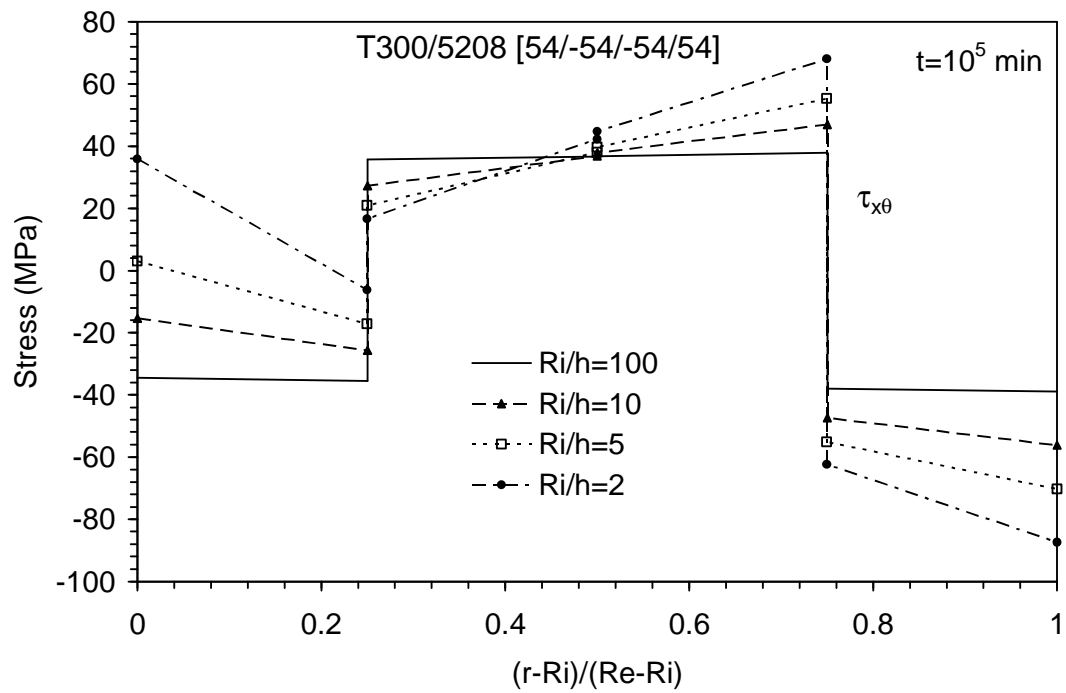
Figure 21: Shear stress distribution at the instant t=10^5 min for cylinders [54/-54/-54/54] under axial compressive load with inner radius to thickness ratios R_i/h of 100, 10, 5 and 2.
