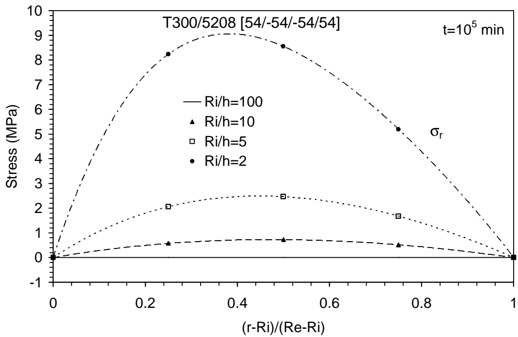
Figure 19: Radial stress distribution at the instant t=10^5 min for cylinders [54/-54/-54/54] under axial compressive load with inner radius to thickness ratios R_i/h of 100, 10, 5 and 2.
