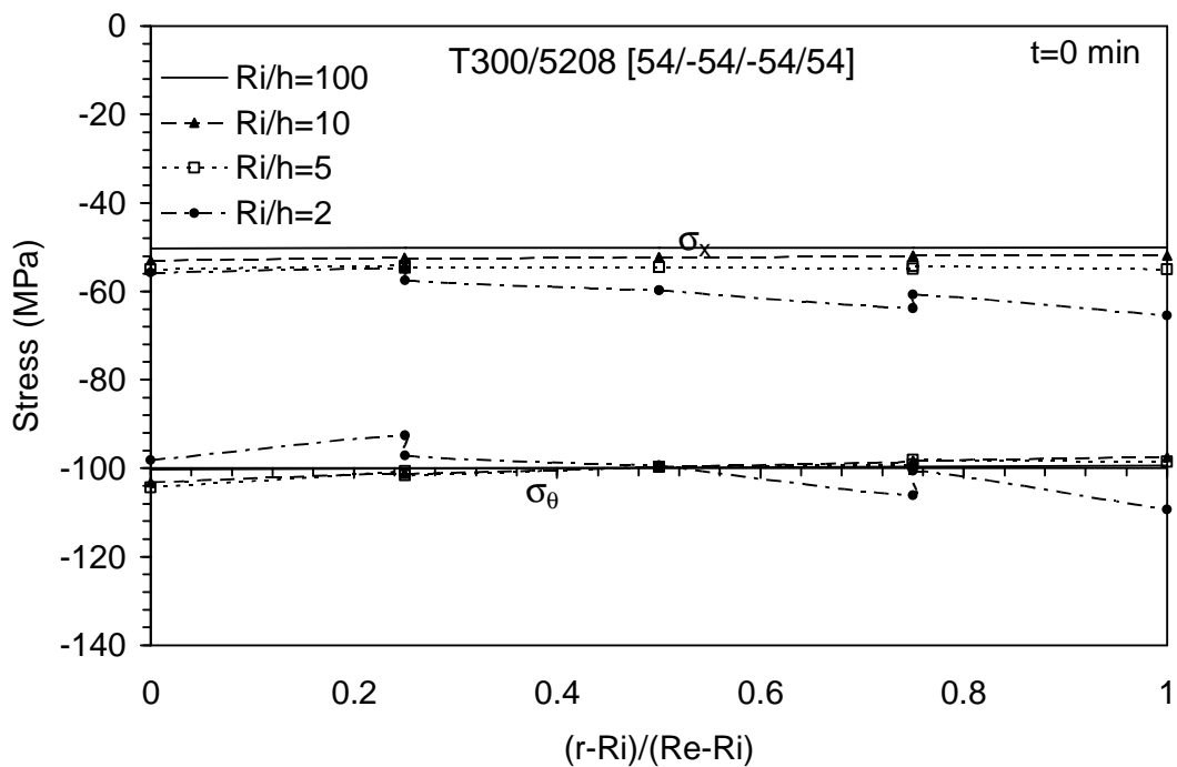
Figure 13: Axial and hoop stress distribution immediately after loading ( t=0 ) for cylinders [54/-54/-54/54] under external pressure with inner radius to thickness ratios R_i/h of 100, 10, 5 and 2.
