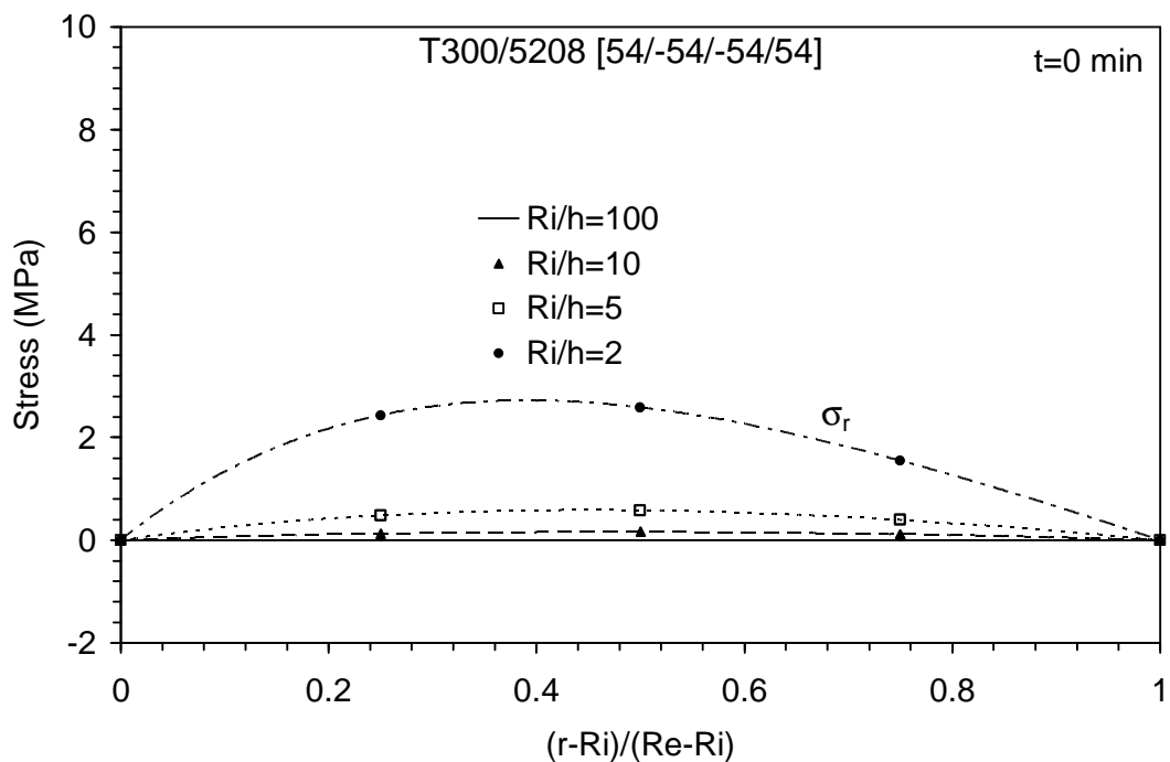
Figure 18: Radial stress distribution immediately after loading ( t=0 ) for cylinders [54/-54/-54/54] under axial compressive load with inner radius to thickness ratios R_i/h of 100, 10, 5 and 2.
