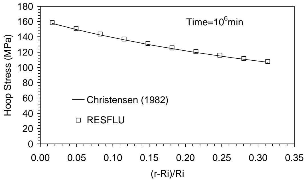
Figure 3: Hoop stress in the viscoelastic material after 10^6 min.
