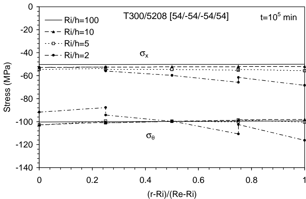
Figure 14: Axial and hoop stress distribution at the instant t=10^5 min for cylinders [54/-54/-54/54] under external pressure with inner radius to thickness ratios R_i/h of 100, 10, 5 and 2.
