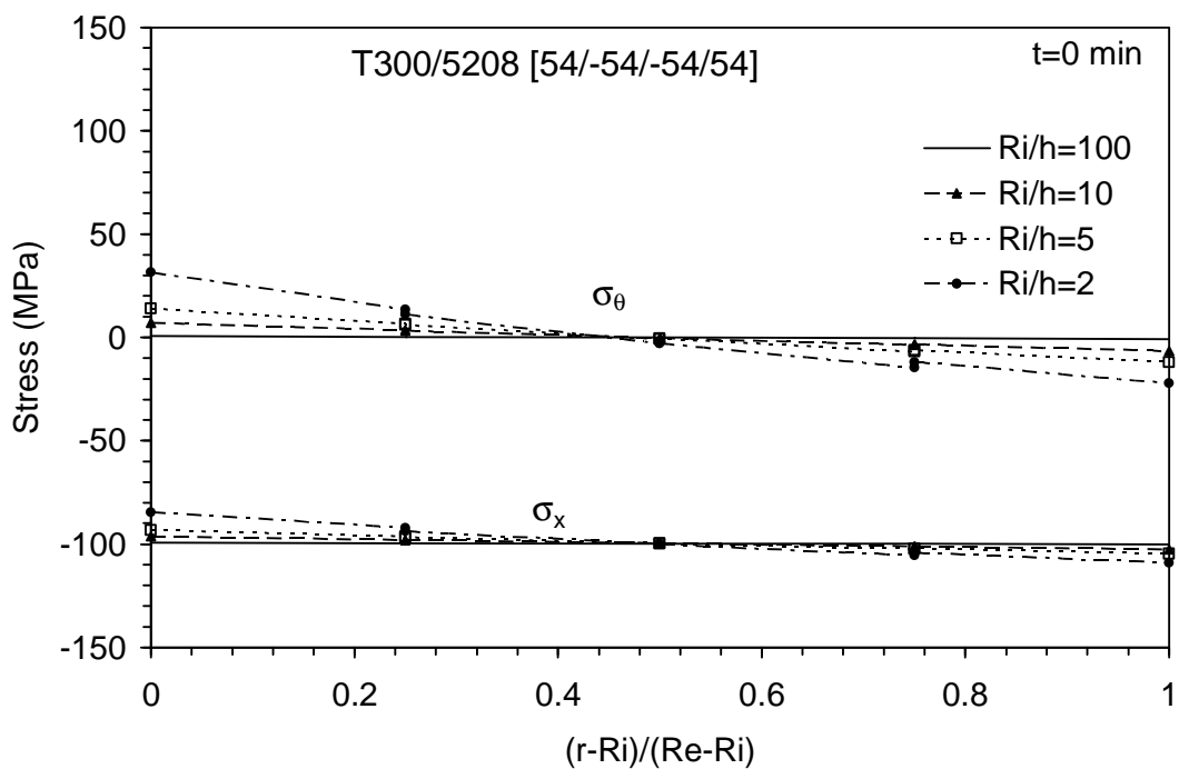
Figure 16: Axial and hoop stress distribution immediately after loading ( t=0 ) for cylinders [54/-54/-54/54] under axial compressive load with inner radius to thickness ratios R_i/h of 100, 10, 5 and 2.
